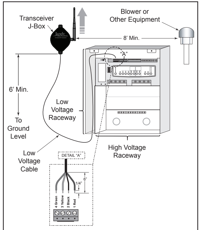
Figure 30. Outdoor Transceiver J-box Installation
