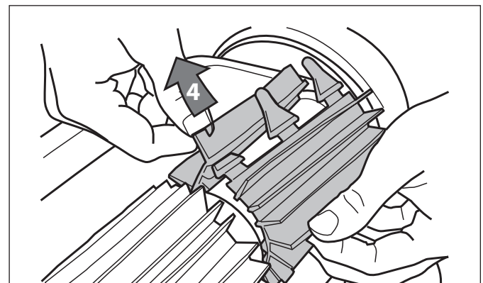
Figure 29. Pull Tabs Through Each Slot
