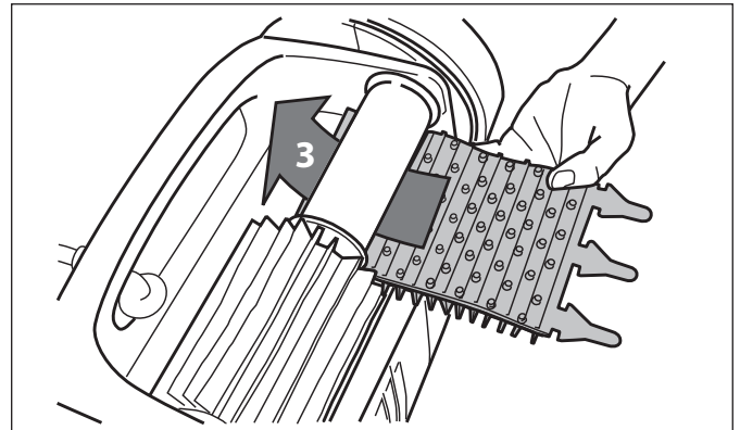
Figure 28. Install the New Brush
