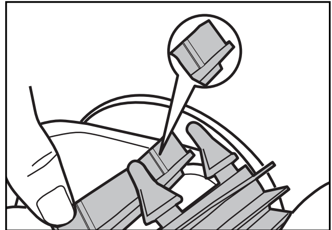
Figure 14. Wear Indicators
